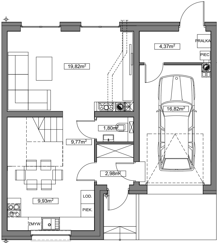
parter, skala 1:100
