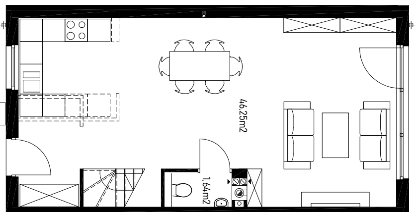
parter 1:100
