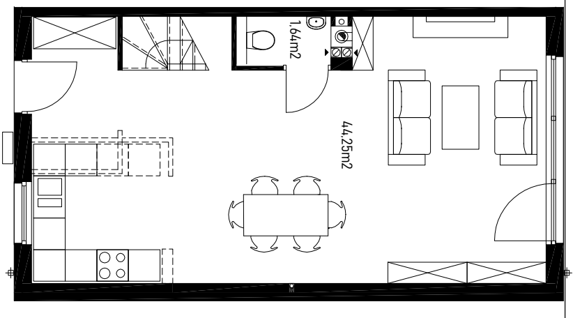
parter 1:100
